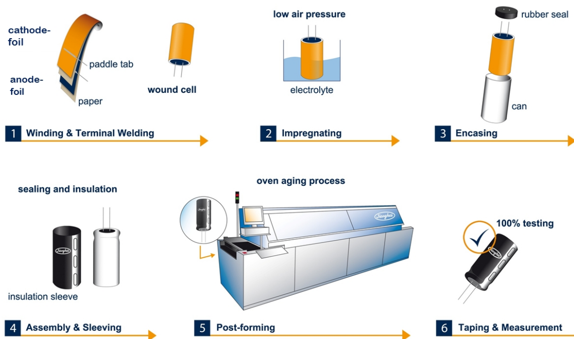
Fig. 3: Process steps from the pre-material to the capacitor
