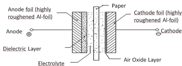
Fig. 1: Construction of an aluminum electrolytic capacitor
