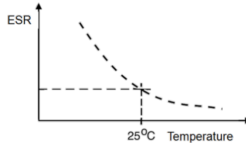
Fig. 3(b): ESR vs. Temperature
