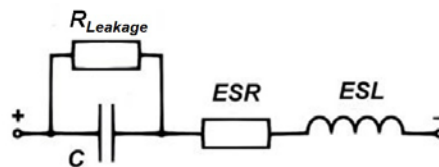
Fig. 2: Equivalent circuit of an elcap
