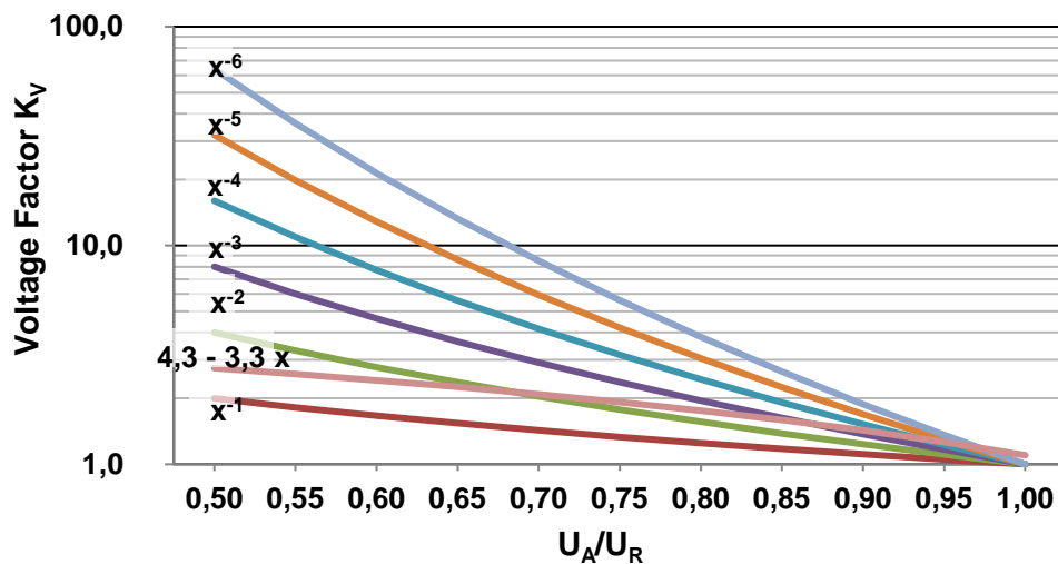
Fig. 8: Voltage factors of various suppliers [4]
