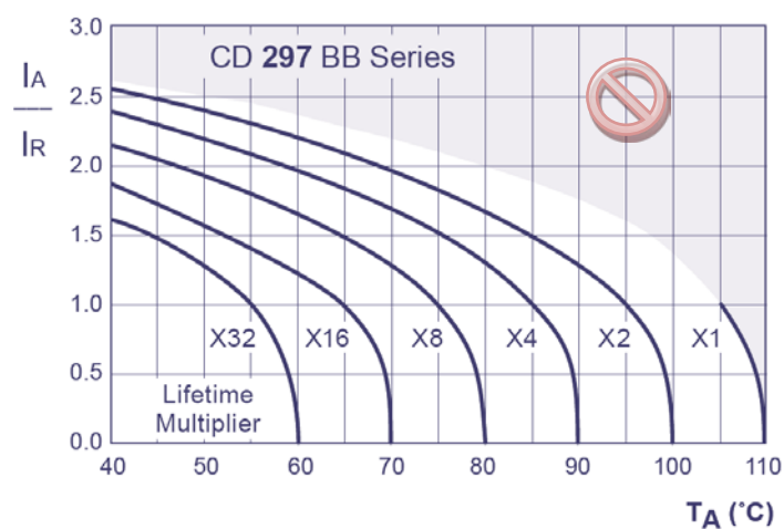
Fig. 7: Lifetime diagram for Jianghai elcap series CD_297_BB
