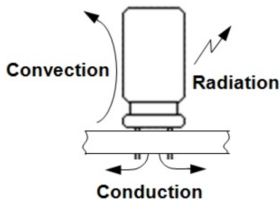
Fig. 4: Cooling mechanisms of elcaps
