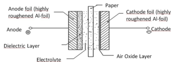
Fig. 1: Internal construction of an Elcap
