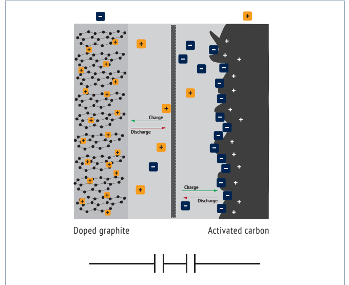
Fig. 3: Electrode structure of LiC
