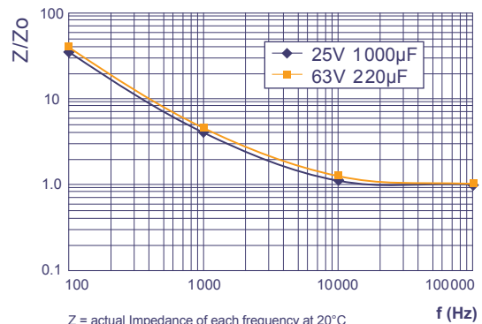
Impedance Ratio
