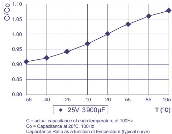
Capacitance Ratio
